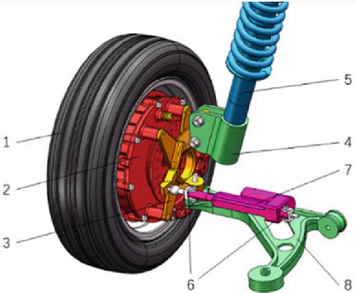
Electric wheel module. 1. Wheels, 2. Hub motor, 3. Steering knuckles, 4. Shock absorber connectors, 5. Spring damping shock absorber, 6. Pusher connection, 7. Electric actuator, 8. Lower control arm
